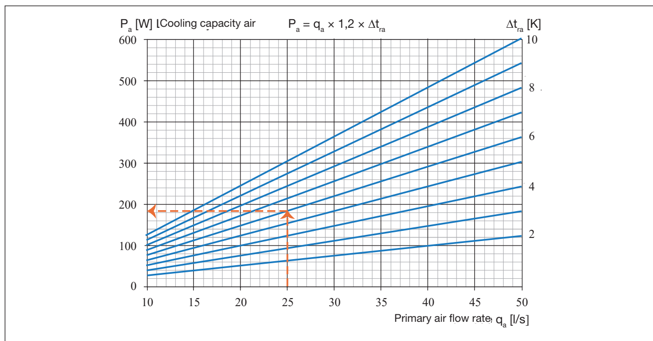
Diagram 1. Luftens kyleffekt P_a som funktion av primärluftflöde q_a . If the air supply flow is 25 l/s and the temperature difference of the room air and the supply air is \Delta t_{ra} = 6 K, then the Cooling capacity of the air is 180 W.
