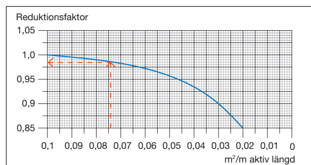
Diagram 5. Effektreducering pga minskad inloppsspalt.
