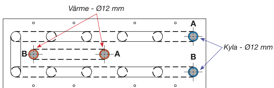
Figur 4. Fasadium: 1000, 1200, 1500.
