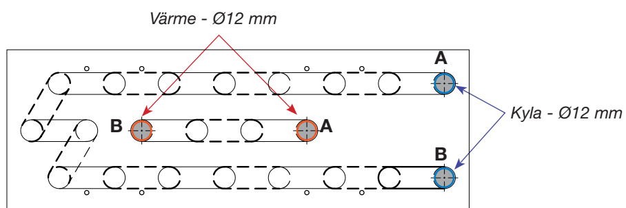
Figur 3. Fasadium: 600, 700, 800.
